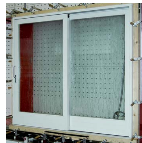
Climatch Lift & Slide door and window during water resistance test.
