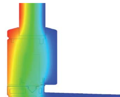
Calculation of heat transmittance coefficient for Climatch Lift & Slide door and window.
